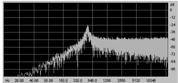
High-pass 12 dB/octave
