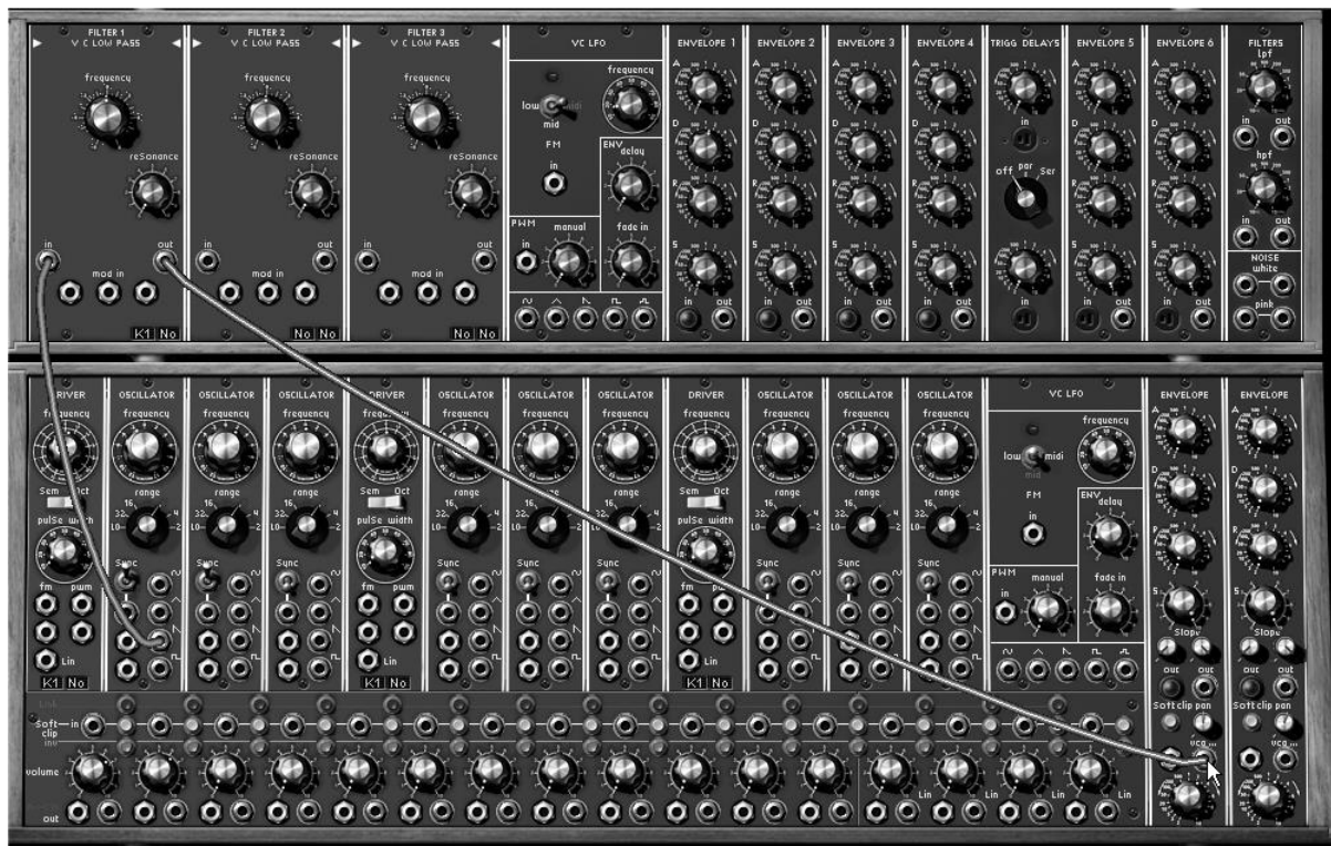
Simple patch #1
