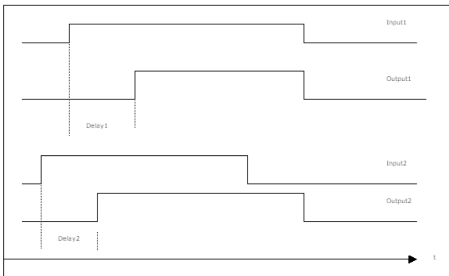
Independent mode
