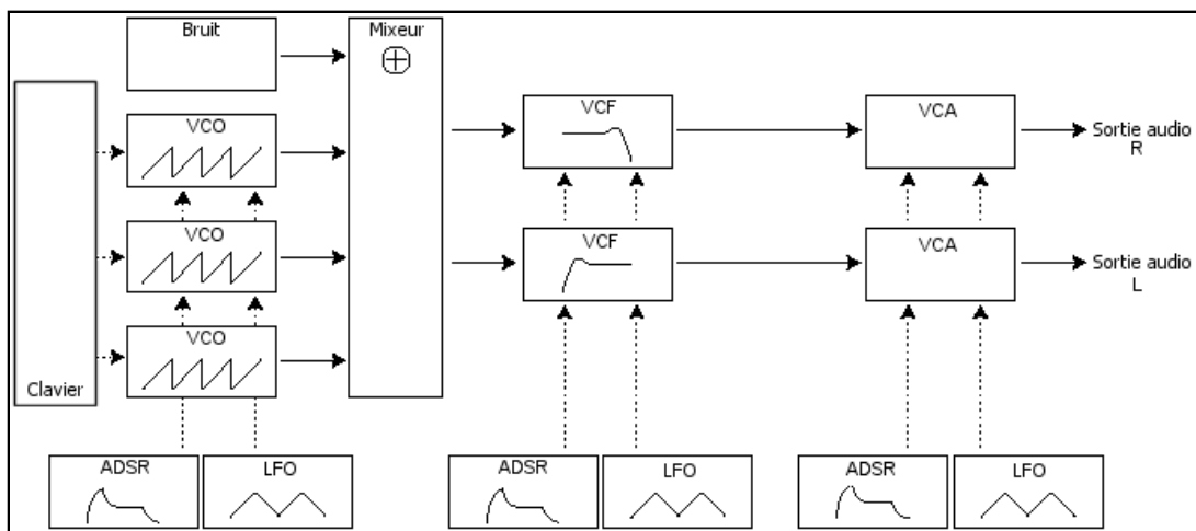
Synthesizer scheme
