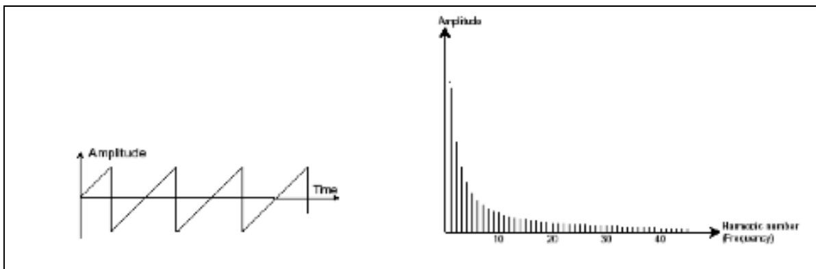
Sawtooth waveform
