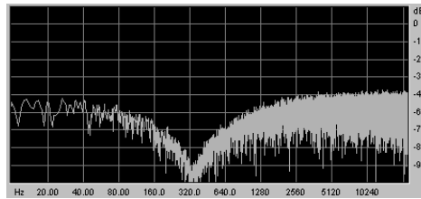
Band reject 24 dB/octave filter
