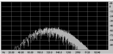
Band-pass 24 dB/octave filter
