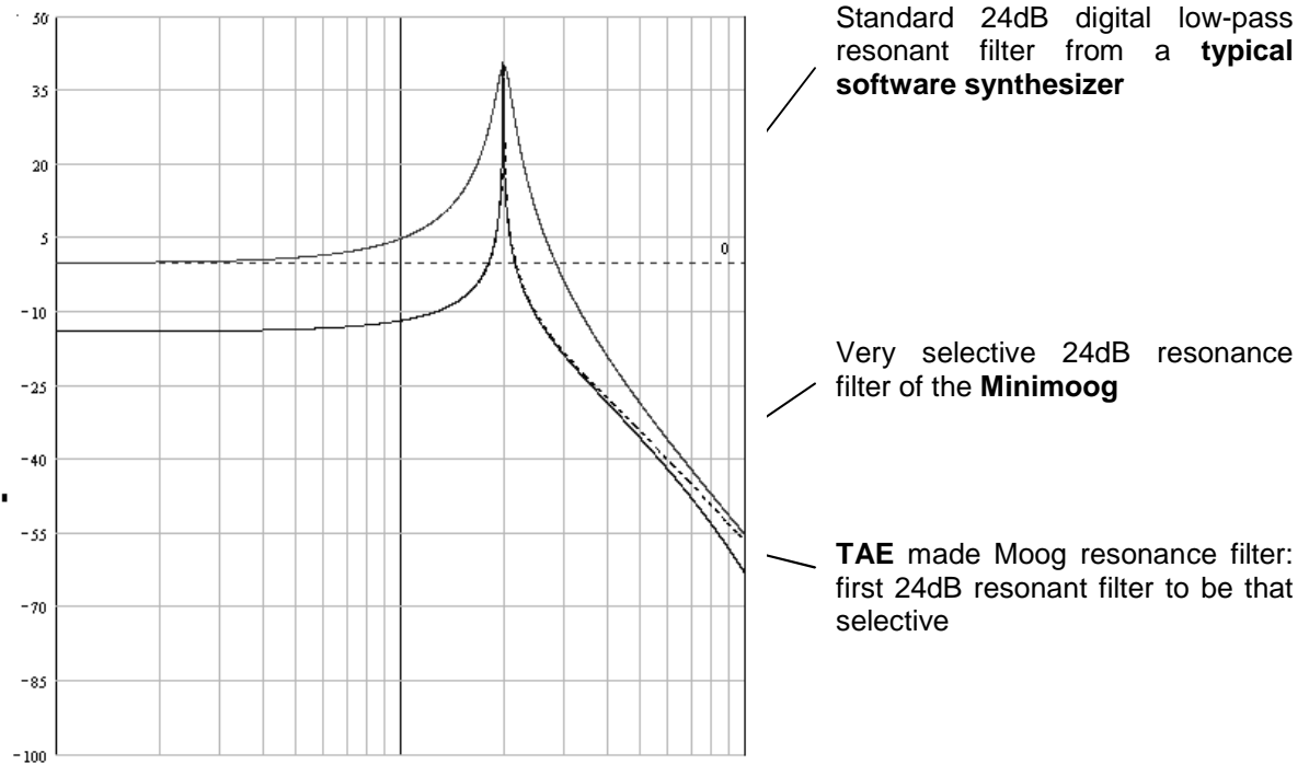
Comparative response filters
