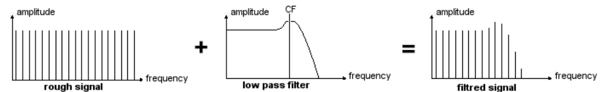
Spectral representation of a rough then 24dB LP filtered signal
