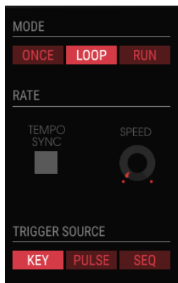
Trigger-Modi
