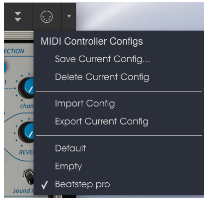
MIDI-Controller Konfiguration
